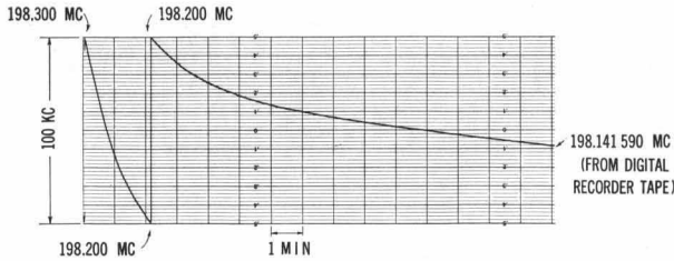
Fig. 3. Curve of warm-up characteristic of oscillator operating near 200 mc. Curve made by operating strip recorder from new digital recorder and -hp- 524B with 525B converter.
